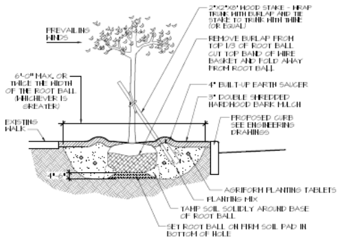
① TREE PLANTING DETAIL NO SCALE
