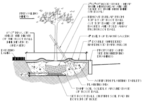
② TREE PLANTING DETAIL NO SCALE (NO SIDEWALK)
